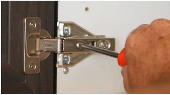
Front screw adjusts door right and left.
